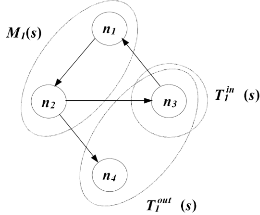
Figure 2.5 The sets T_1^{\text{out}}(s) and T_1^{\text{in}}(s) relative to M_1(s) = \{n_1, n_2\} [Cordella, et al., 1999].
