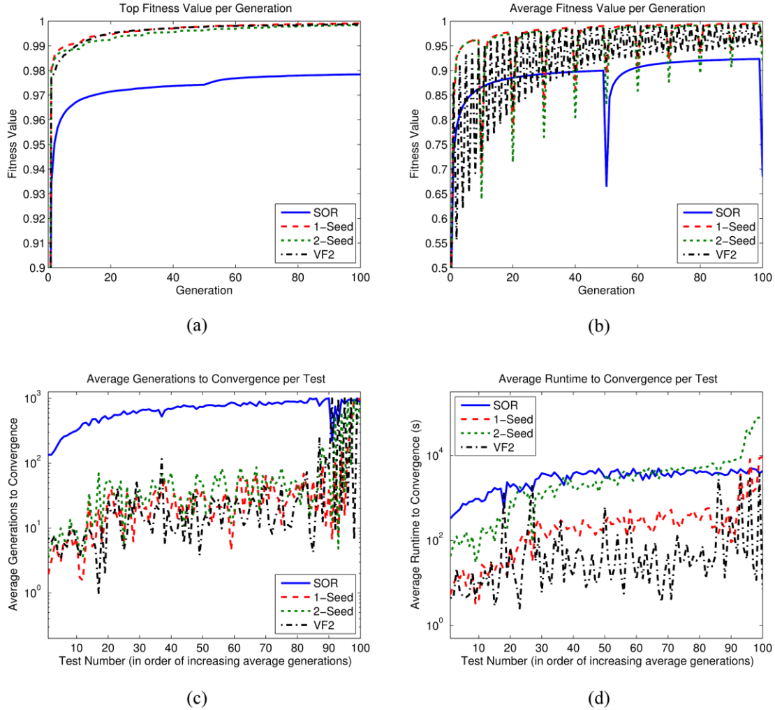
Figure 4.6 Results of the experiments with simplified sketches. (a) Top fitness value per generation. (b) Average fitness value per generation. (c) Average generations to convergence per test. (d) Average runtime to convergence per test.
