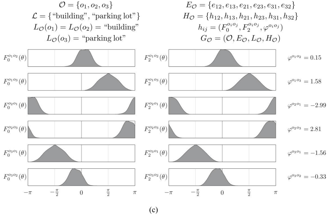
Figure 3.2 ARG representation of an object set. (a) An example of an object set \mathcal{O} = \{o_1, o_2, o_3\} (b) The ARG representation of the object set. (c) Formal definition of G_{\mathcal{O}} and its attributes.
