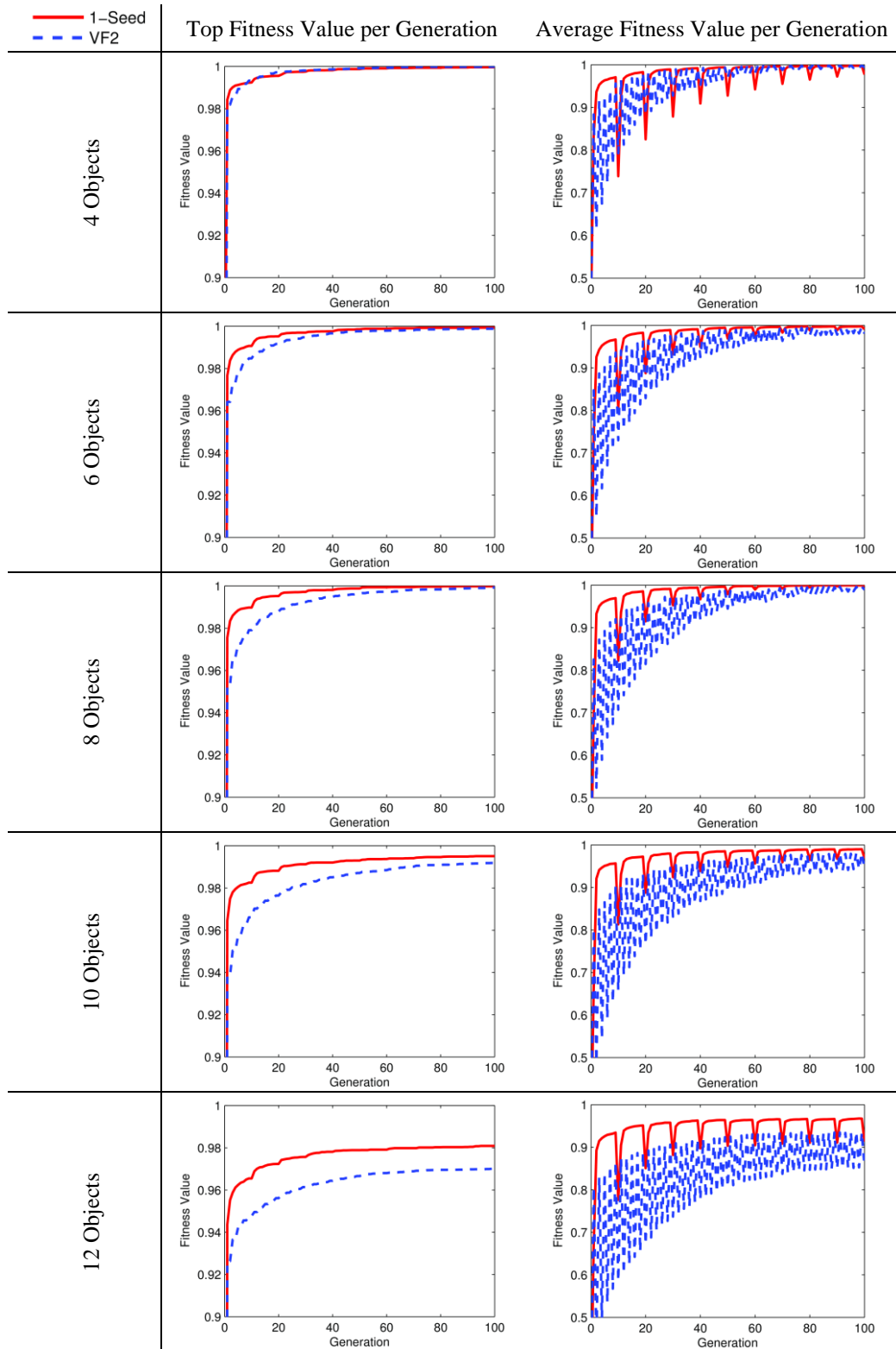
Figure 4.8 Impact of sketch size on fitness values for resubstitution sketches.
