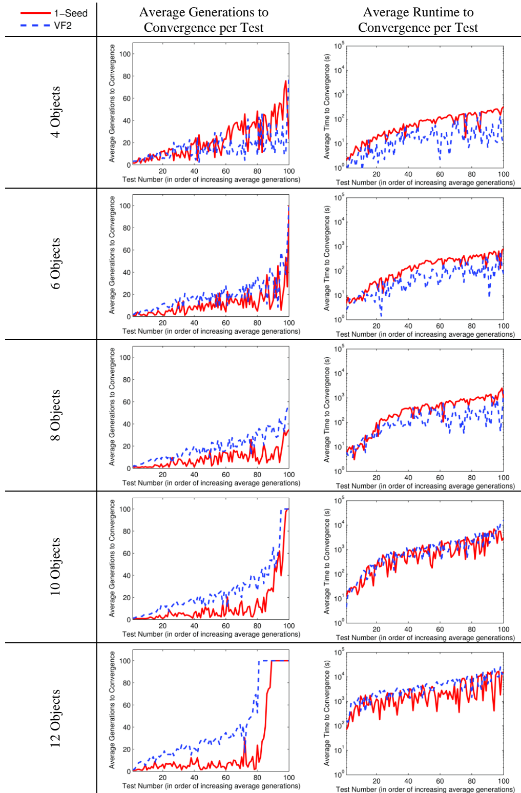
Figure 4.9 Impact of sketch size on convergence time for resubstitution sketches.
