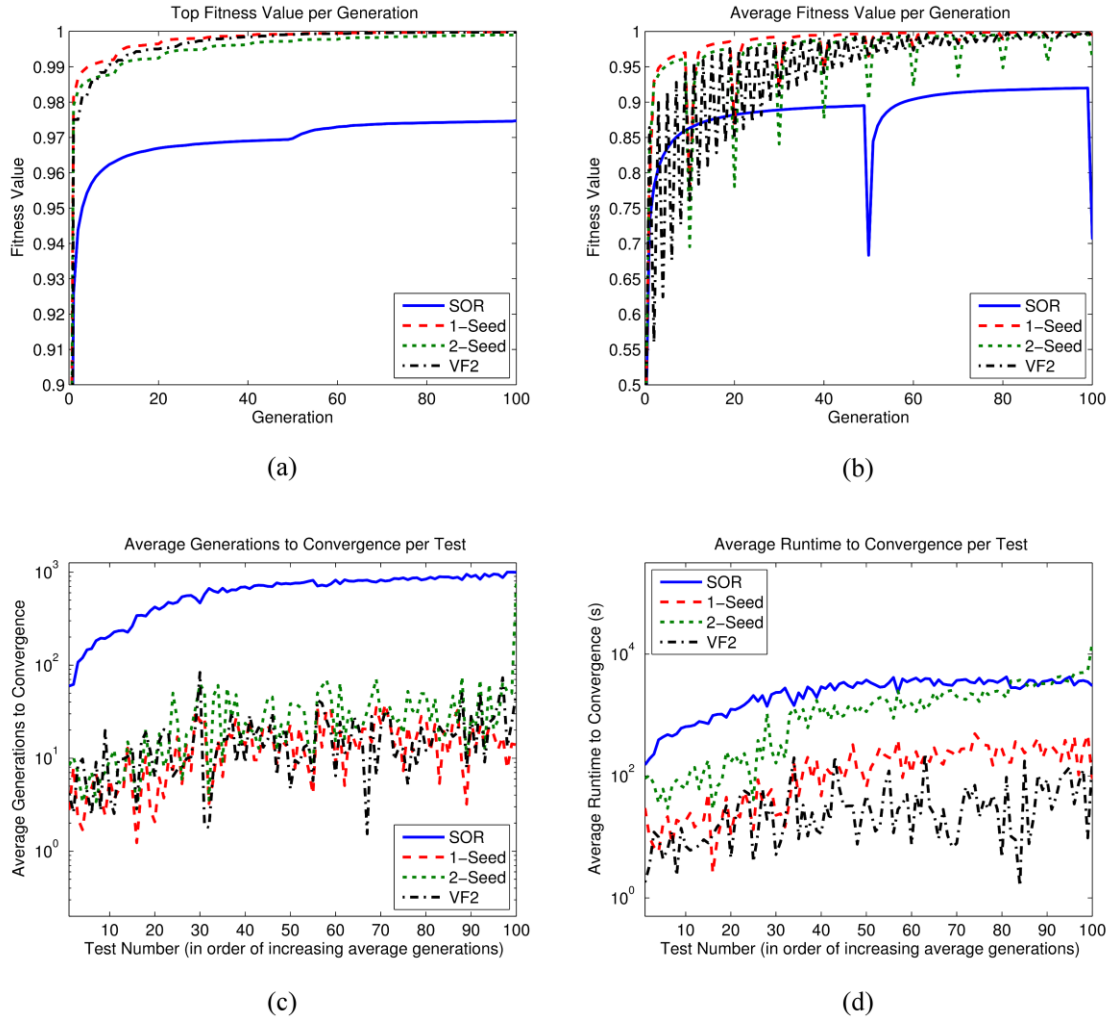
Figure 4.4 Results of the resubstitution experiments. (a) Top fitness value per generation. (b) Average fitness value per generation. (c) Average generations to convergence per test. (d) Average runtime to convergence per test.
