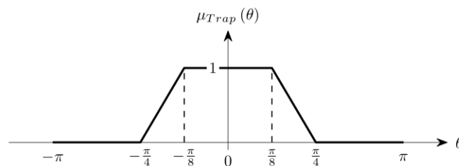
Figure 3.4 The trapezoidal weighting function used for elastic angles.
