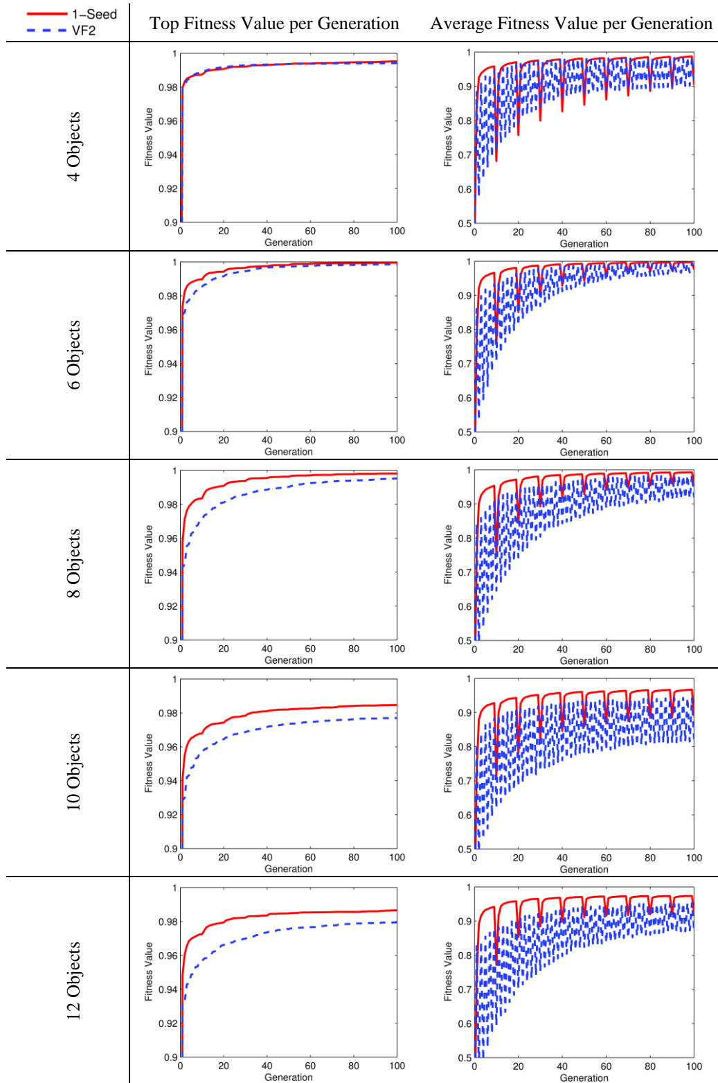
Figure 4.10 Impact of sketch size on fitness values for simplified sketches.
