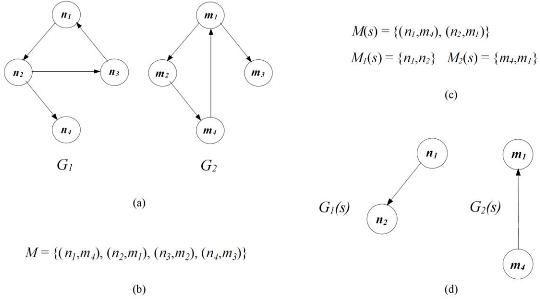
Figure 2.3 Example of the partial mapping function used in the VF algorithm [Cordella, et al., 1999]. (a) Two graphs G_1 and G_2 . (b) The only possible mapping M . (c) A partial mapping solution M(s) and the corresponding partial node sets M_1(s) and M_2(s) . (d) The corresponding subgraphs G_1(s) and G_2(s) .
